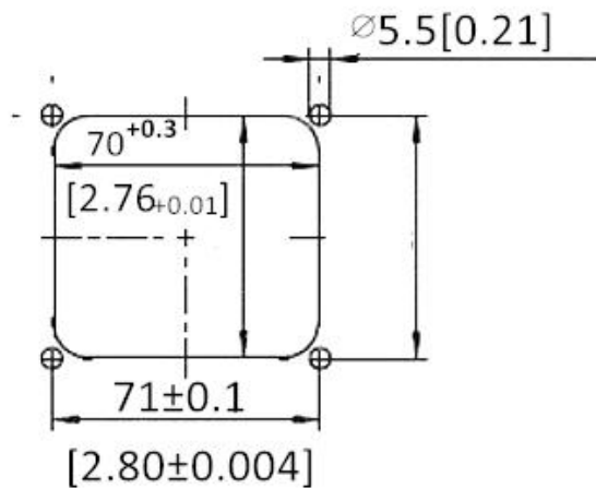
INSTALL DIMENSIONS
